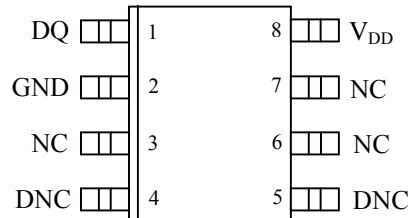
DS1821S 8-Pin SOIC (208-mil) See Mech Drawings Section
